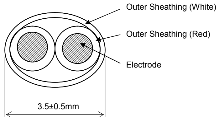
Fig. 2: Cross-section Diagram of the AD-RS Sensor
