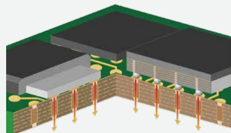
Thermal release
