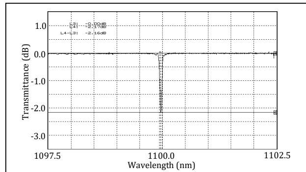
A sample of 1100nm FBG
